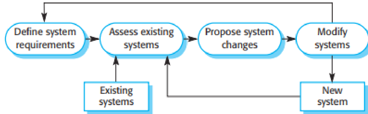
Fig: Software system Evolution
